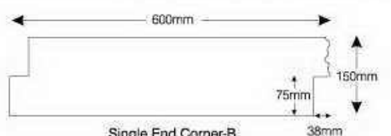
Single End Corner-B
