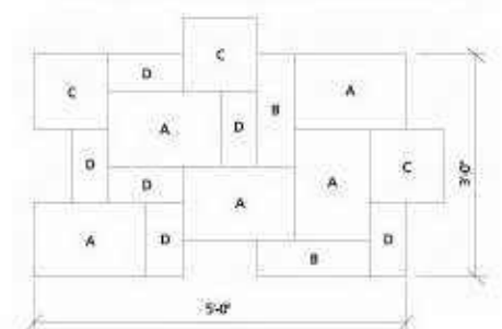
B81 Interlocking Unit Lays Out 5'-0" x 3'-0" or 15 Square Feet
