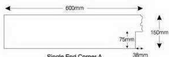
Single End Corner-A
