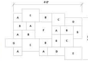
B80 Interlocking Unit Lays Out 4'-0" x 2'-6" or 10 Square Feet
