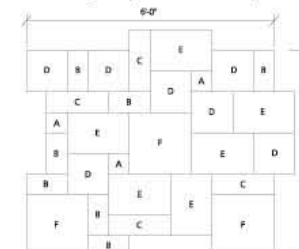
B83 Interlocking Unit Lays Out 6'-0" x 5'-0" or 30 Square Feet
