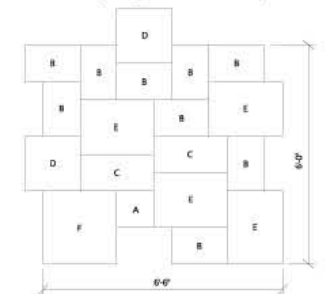
B84 Interlocking Unit Lays Out 6'-6" x 6'-0" or 39 Square Feet
