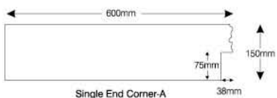
Single End Corner-A
