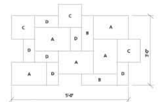
B81 Interlocking Unit Lays Out 5'-0" x 3'-0" or 15 Square Feet
