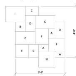
B82 Interlocking Unit Lays Out 4'-0" x 3'-9" or 15 Square Feet
